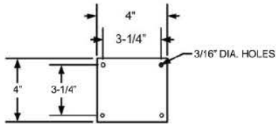
Mounting Plate Dimensions and Hole Locations
